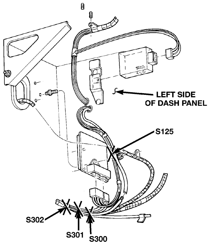
Fig. 5 Body Splices—RHD
