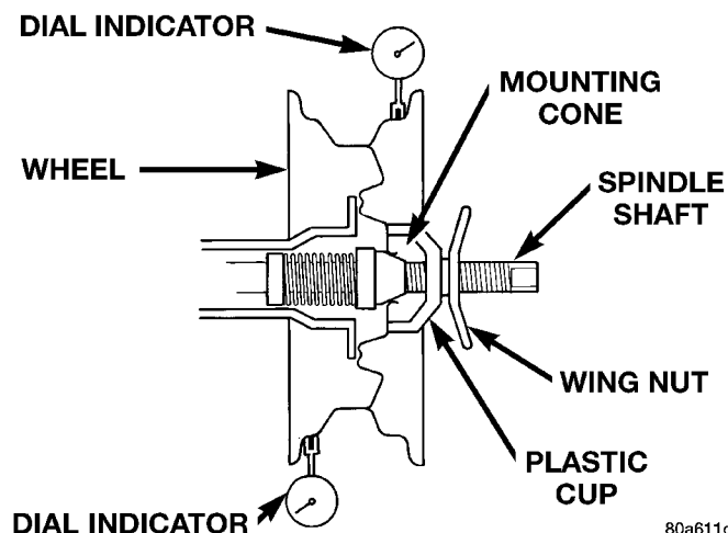
Fig. 3 Radial Runout
