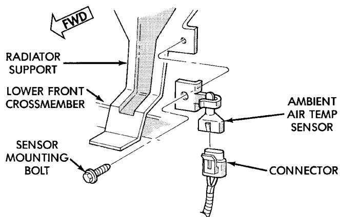
Fig. 6 Ambient Temperature Sensor Remove/Install
