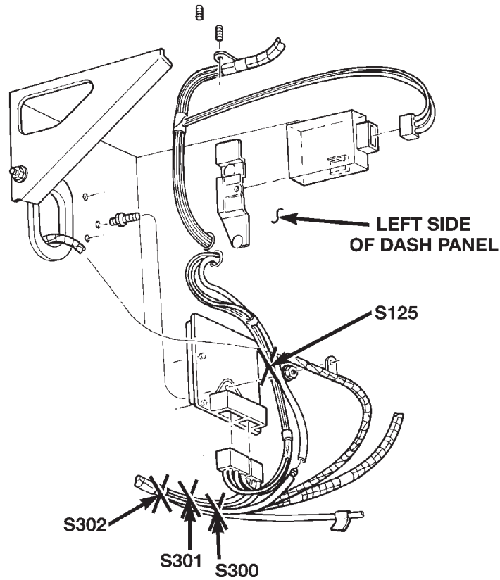
Fig. 5 Body Splices
