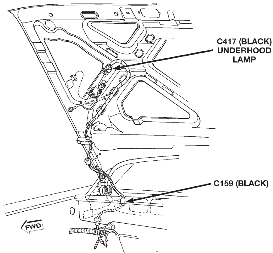
Fig. 22 Underhood Lamp
