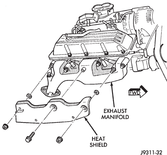
Fig. 16 Exhaust Manifold Heat Shields (Left Shield Shown)
