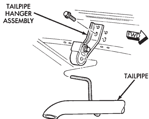
Fig. 10 Tailpipe Hanger
