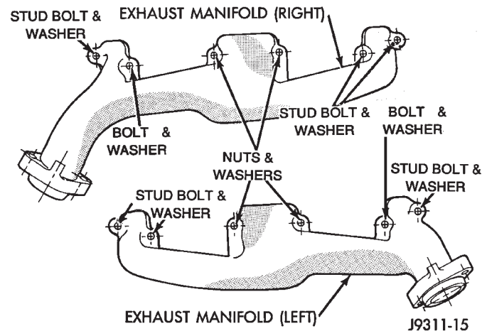
Fig. 17 Exhaust Manifold
