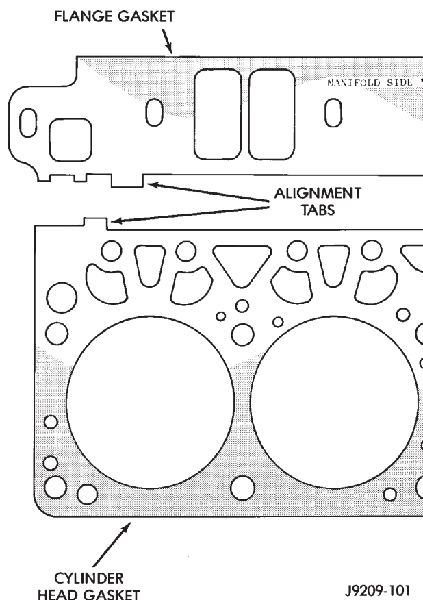
Fig. 14 Intake Manifold Flange Gasket Alignment
