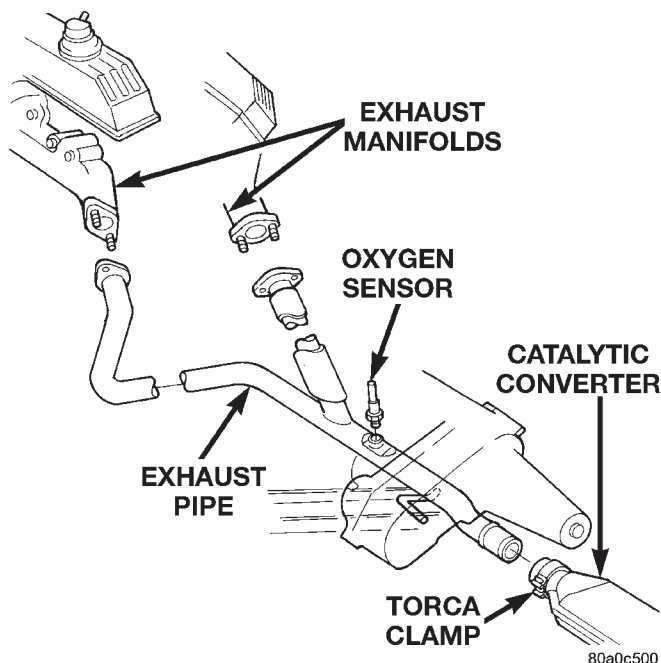
Fig. 7 Exhaust Pipe—5.2L Engine
