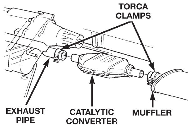
Fig. 9 Exhaust Pipe-to-Catalytic Converter-to-Muffler Connection
