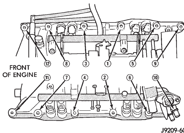
Fig. 15 Intake Manifold Bolt Tightening Sequence
